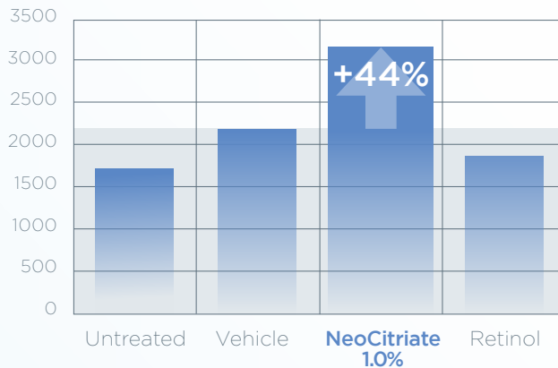
Effect on Type 1 Collagen Synthesis in Human Fibroblast Cell Culture Media
